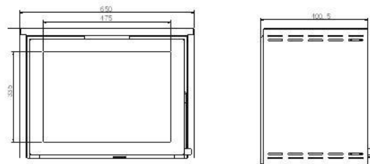
Unit Dimensions without frame 650 wide x 400 deep x 510 high
