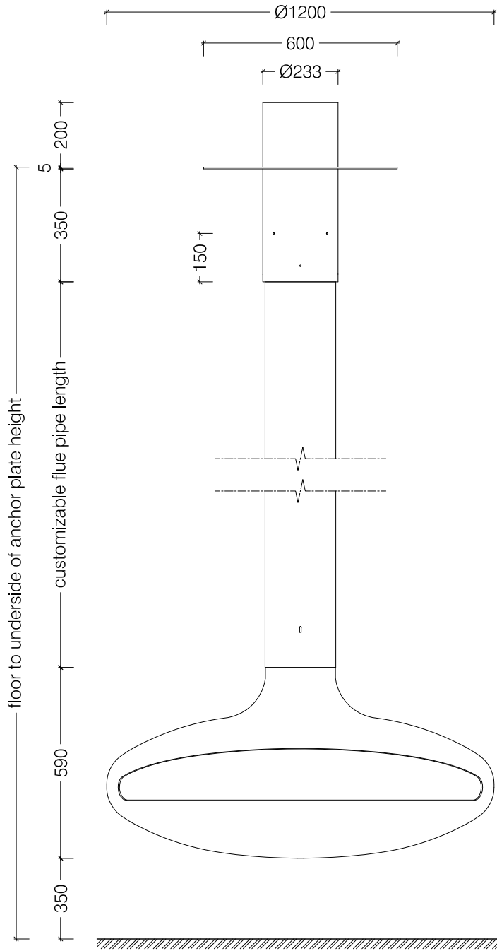
Front View
